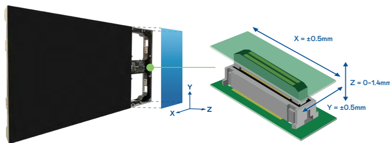
LED modules adjustable in X, Y, Z directions
